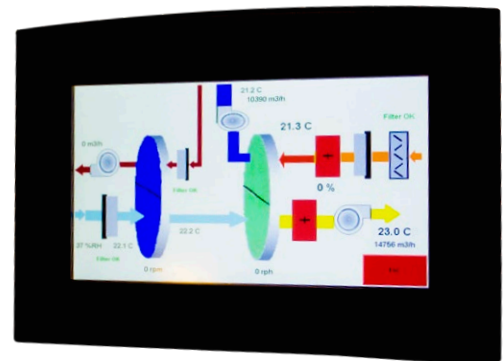
PLC C7 with graphic touch display, 7". Advanced PLC control and possible to add Profibus communication
