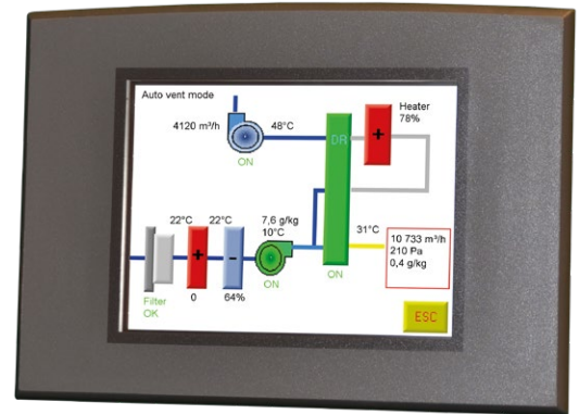
PLC C4 with graphic touch display, 5.7". Advanced PLC control with great expansion options
